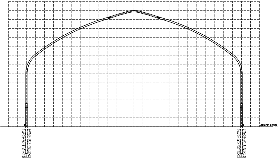
A 3 6'-0" SIDEWALLS EACH BLOCK = 1'-0"x1'-0"
